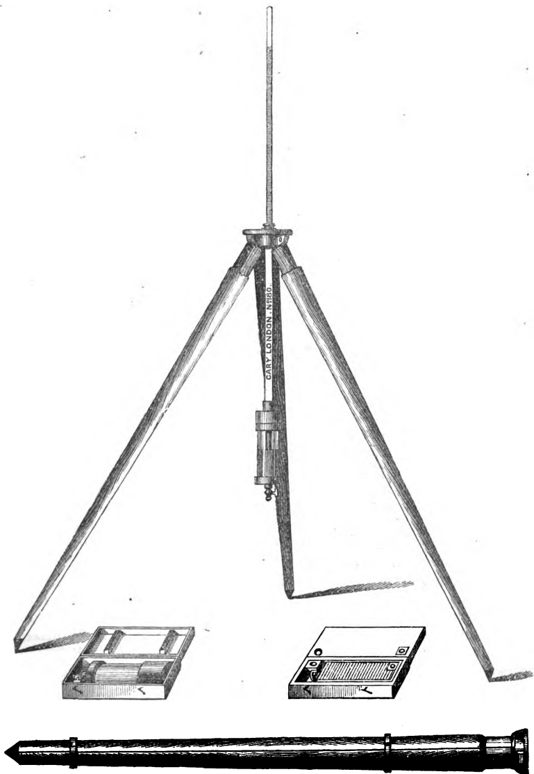
GEORGE'S MERCURIAL BAROMETER.
