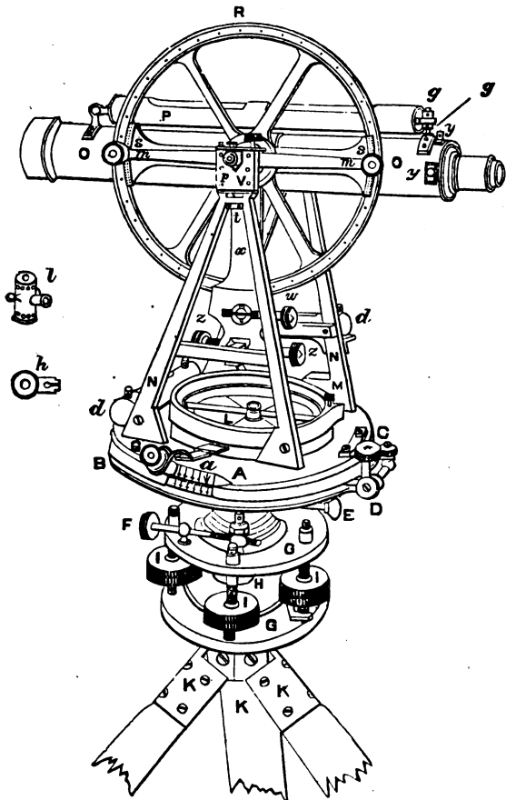
TRANSIT THEODOLITE.
