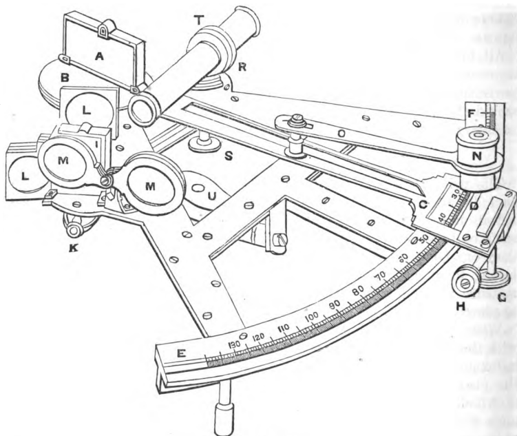
SEXTANT.
