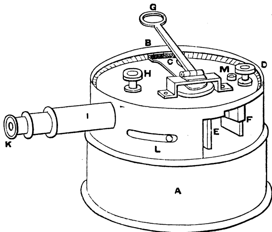
BOX SEXTANT.
